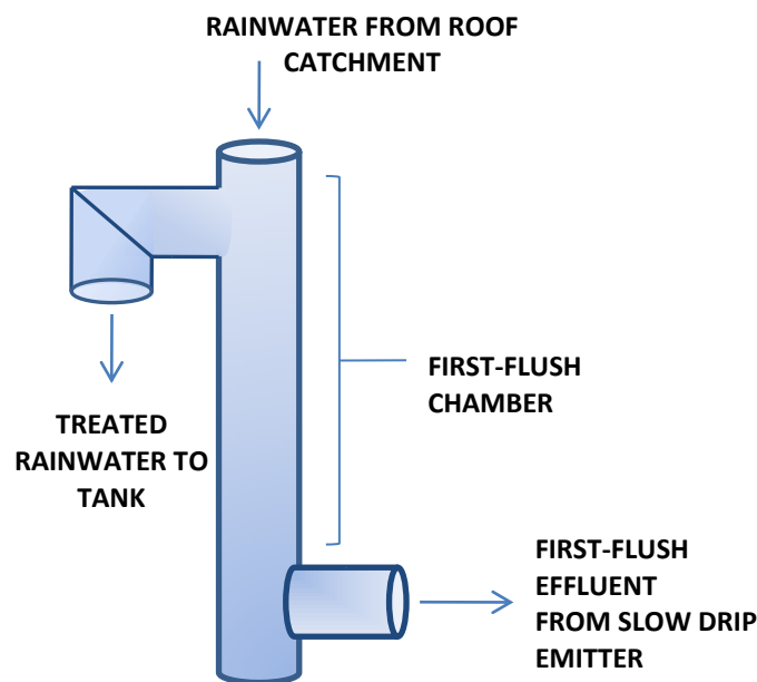
Figure 3-2. Schematic indicating the operation of a first-flush diverter
