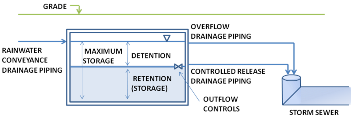
Figure 6-2. Schematic of RWH system with outflow controls and controlled release drainage piping for stormwater management. ('DETENTION' is the volume of runoff to be slowly released to storm sewer. The remaining volume 'RETENTION' is used to supply rainwater to permitted fixtures)
