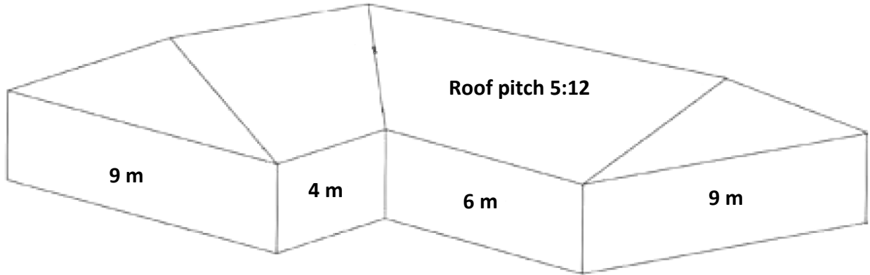
Figure A-1. Roof drainage area to be guttered (isometric 'facing' view) 26
