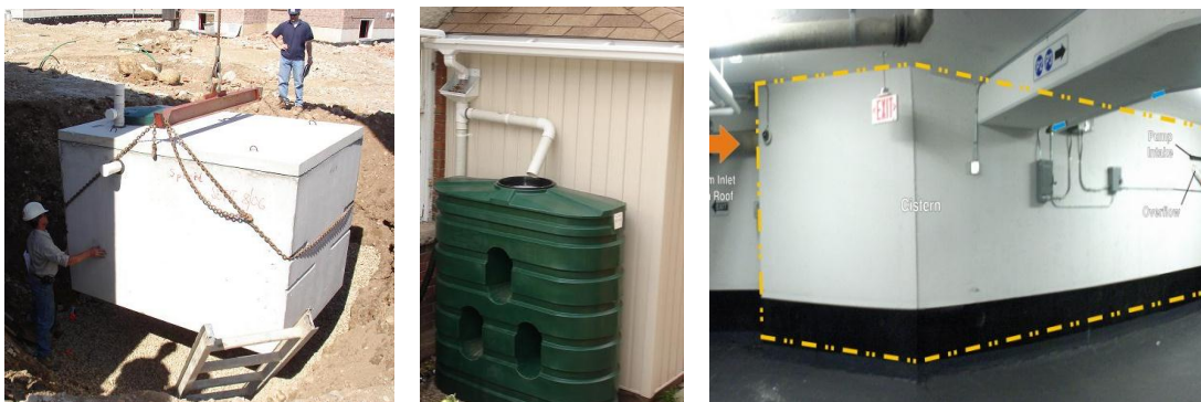
Figure 2-1. [LEFT] Pre-cast concrete tank (below ground application), [CENTRE] Plastic tank (above ground application) and [RIGHT] Cast in place concrete tank integrated within parking garage (integrated storage) 6
