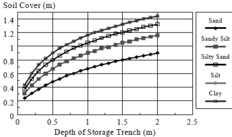
Figure D-3. Soil cover for soakaway pits, based on frost heave 54
