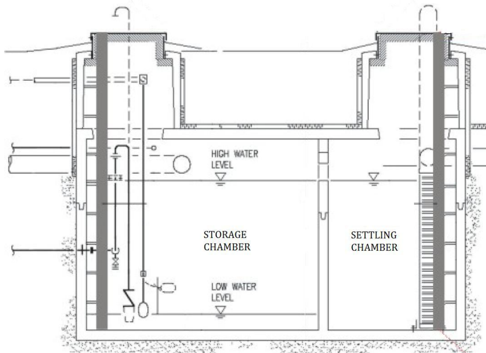
Figure 3-4. Rainwater storage tank with integrated settling and storage chambers 12
