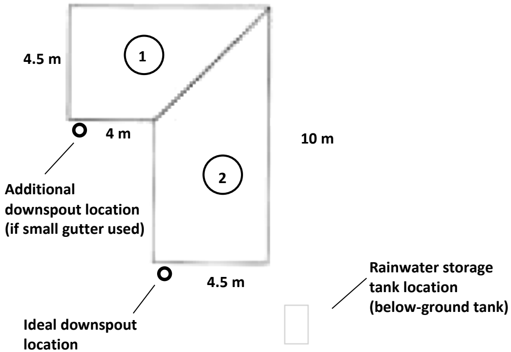
Figure A-2. Roof drainage area to be guttered (projected 'top-down' view) 27
