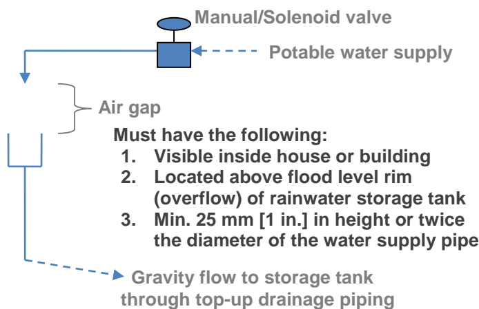
Figure 4-2. Schematic drawing of a top-up system with an air gap 18
