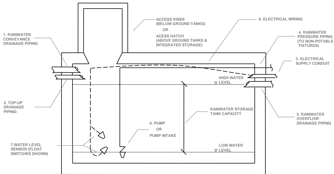
Figure 2-2. Rainwater storage tank schematic
