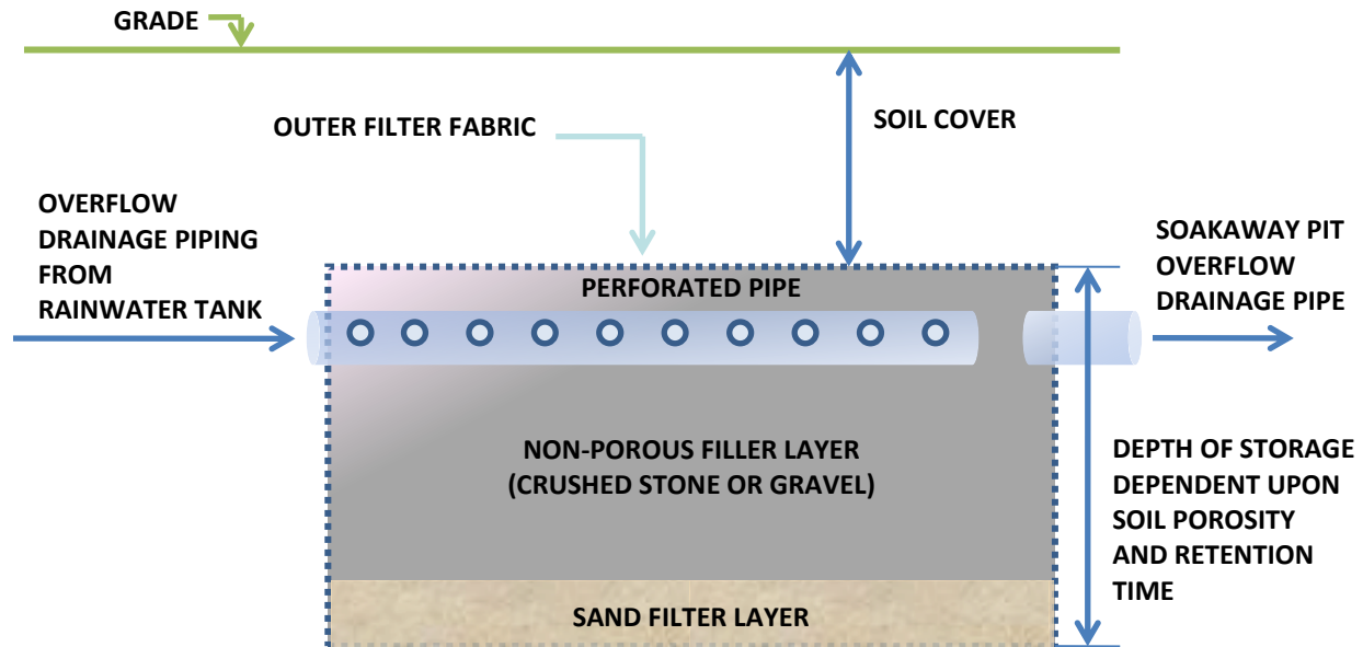
Figure D-2. Sketch of a typical soakaway pit (cross-section view) 50
