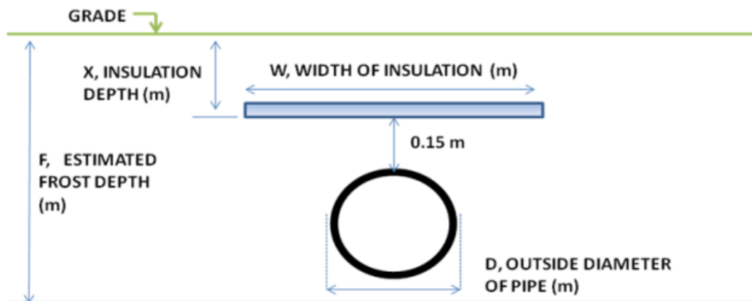
Figure A-5. Frost protection of pipe by horizontal insulation 32
