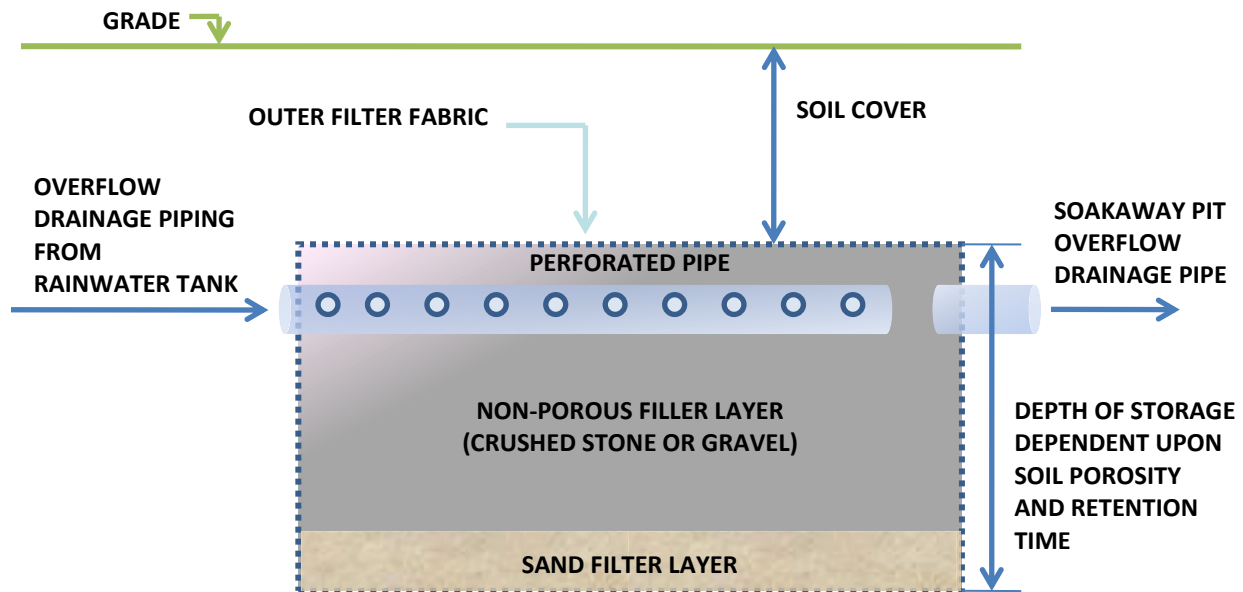
Figure 6-1. Sketch of a typical soakaway pit (cross-section view) 21
